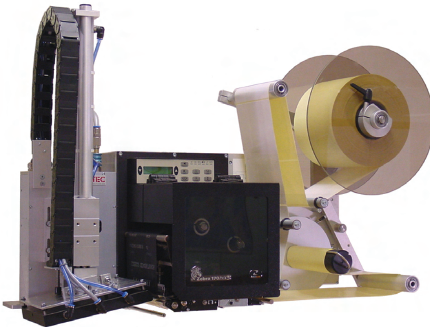
Printer and applicator in right hand version
