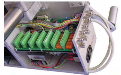
Controller and I/O:s easy accessible
